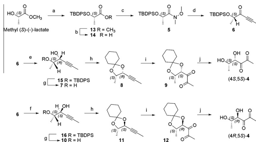
Scheme 3. Synthesis of two isomers of 4,5-dihydroxyhexanedione 4 (DHDs). Reagents and Conditions: (a) TBDPSCI, Et 3 N, DMAP, CH 2 Cl 2 , 92%; (b) LiOH, THF/H 2 O, quant. (c) CH 3 (CH 3 O)NH 2 Cl, CDMT, NMM, THF, 84%; (d) propyne, BuLi, THF, −78 °C, 73%; (e) (S)-Alpine Borane, THF; (f) CeCl 3 ·7H 2 O, NaBH 4 , CH 3 OH, −50 °C; (g) TBAF, THF, 36% 7 and 53% 10 , two steps, dr 0.95 for 7 and 10 ; (h) c -hexanonedimethylacetal, H 2 SO 4 , DMF, 83%; (i) NaIO 4 , cat. RuO 2 ·H 2 O, CH 3 CN/CCl 4 /H 2 O, 46%; (j) H 2 SO 4 0.01 M.
