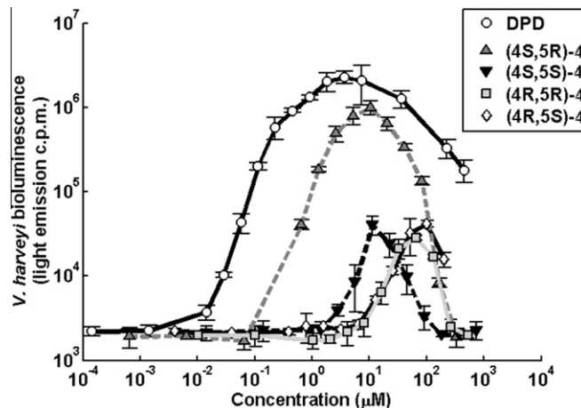
Figure 4. Bioluminescence assay of DPD and C-5 DPD with V. harveyi reporter strain MM32. Error bars indicate standard deviations.
