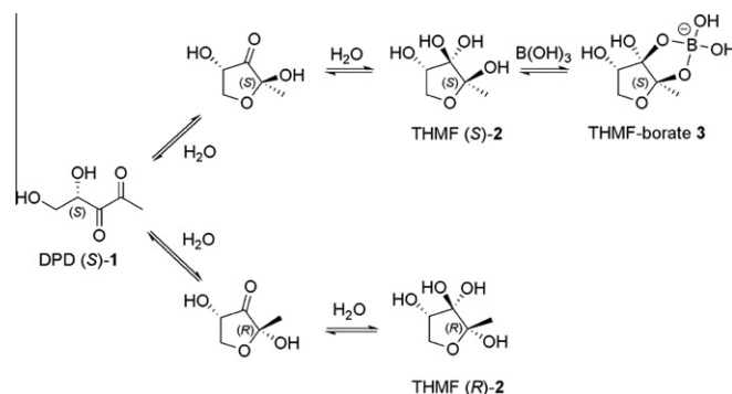
Scheme 1. Forms of AI-2 in water.
